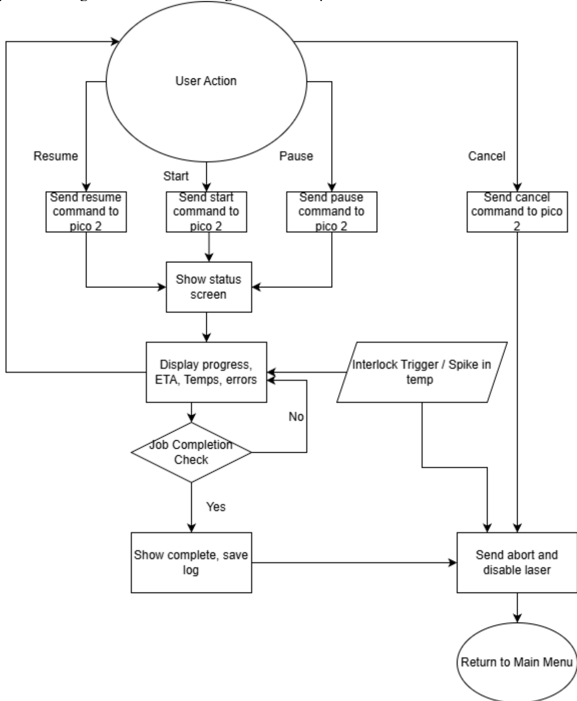
Figure 34: Job Monitoring Flowchart
