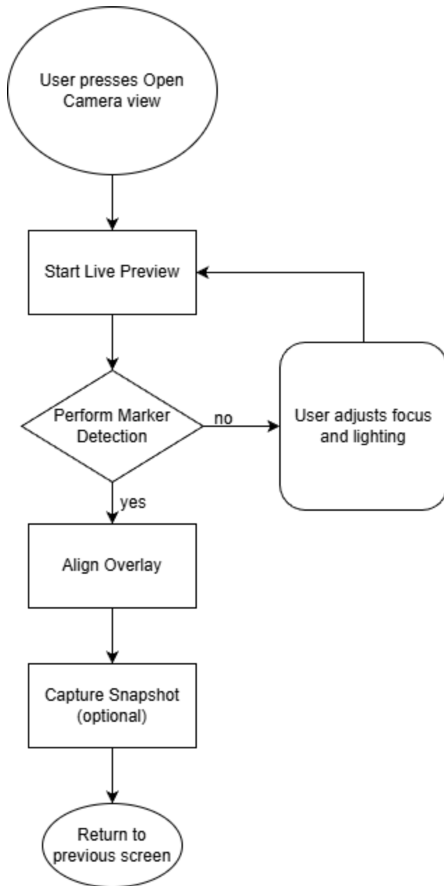
Figure 33: Camera and Alignment Flowchart
