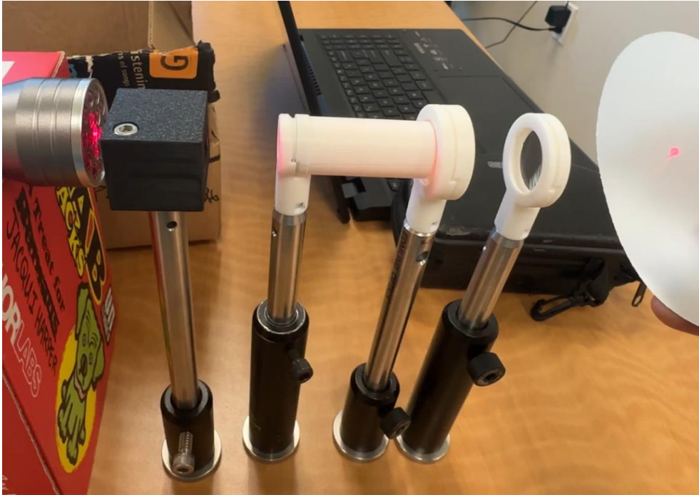
Figure 37: Optical System Testing (Jacqui)
