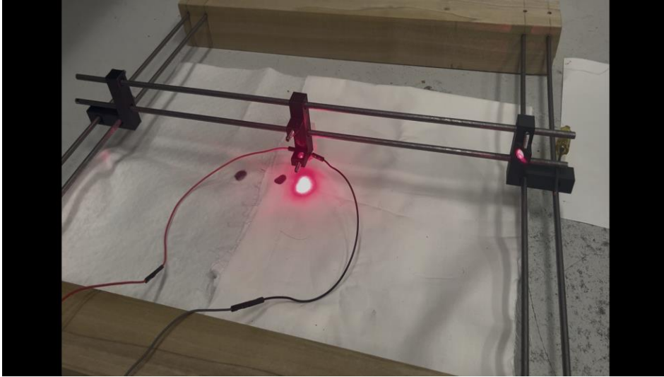
Figure 44: Mirrors guiding beam onto specific spot on the fabric. Fabrics not placed at focal length for demonstration purposes.
