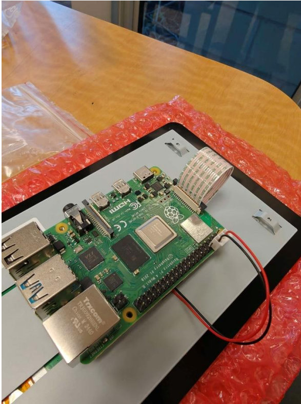
Figure 38: Touch Display 2 to Raspberry Pi 4B Connection
