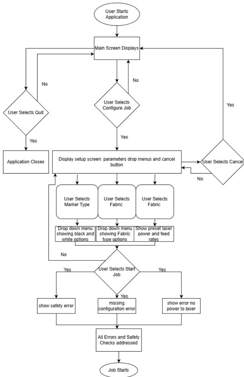
Figure 32: Initiate Job Flowchart
