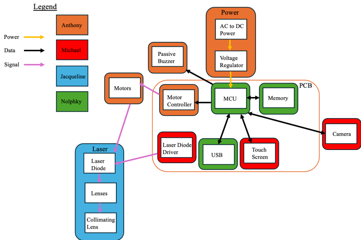
Figure 4: Hardware Block Diagram
