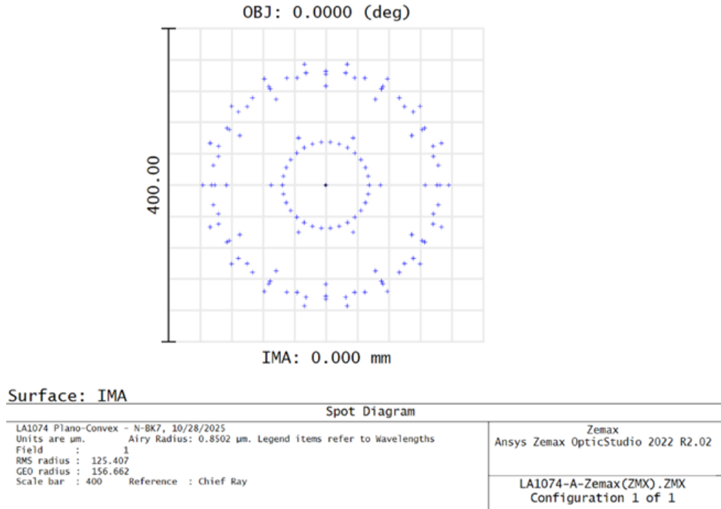
Figure 14: (LA1074-A) Plano-convex 19.6 mm focal length lens, minimum spot size 313.324 \mu\text{m} (Zemax)
